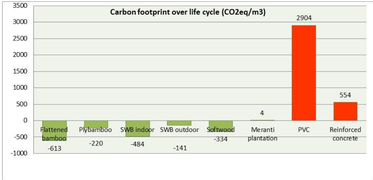
Figure 11: Carbon Footprint over Life Cycle (kgCO 2 eq / m 3 building material) for various common building materials (this report, Idemat 2014 database and Vogtländer et al. 2014). Note: aluminium and steel are not shown because of the high carbon footprint (see table 7) therefore not fitting in the graph.
