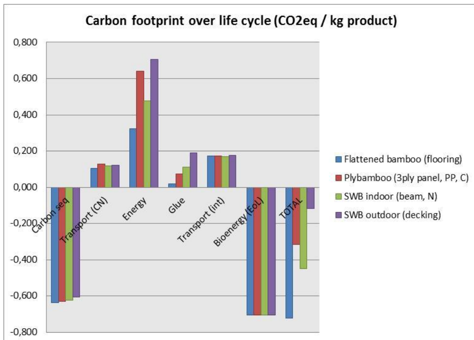
Figure 8: Carbon Footprint over Life Cycle (kgCO 2 eq / kg MOSO product), for various MOSO products based on different production technologies.
