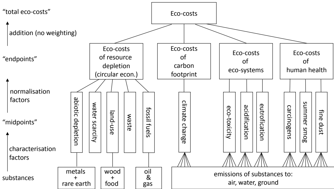
Figure 18: Calculation structure of the eco-costs 2012
