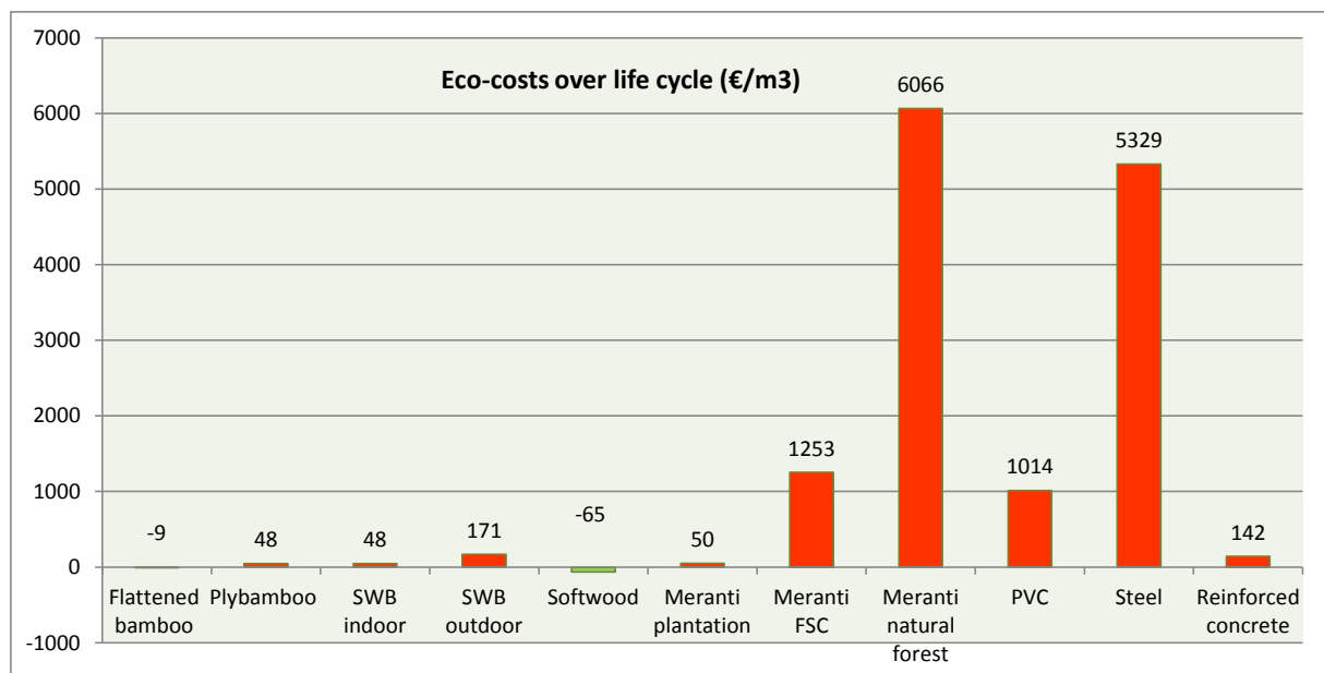
Figure 12: Eco-costs over Life Cycle (€/ m3 building material) for various common building materials (this report, Idemat 2014 database and Vogtländer et al. 2014). Note: aluminium is not shown because of the high eco-costs (see table 8) therefore not fitting in the graph.
