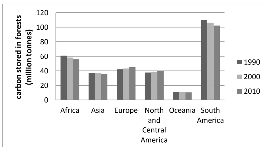
Figure 15: Trends in carbon storage in forests from 1990–2010 (Source: FAO 2010)
