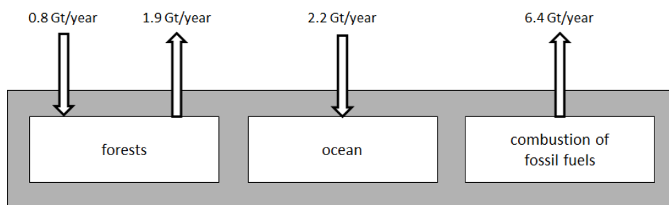
Figure 13: Global anthropogenic fluxes of CO 2 (Gt/year) over the period 2000–2010
